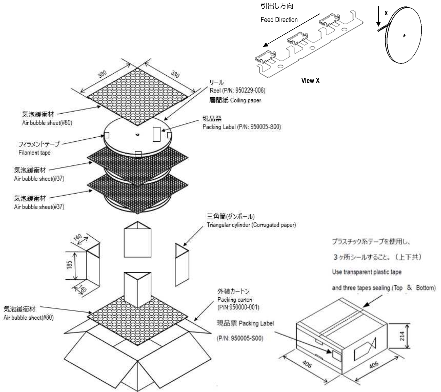
Fig.2 Packing Method
