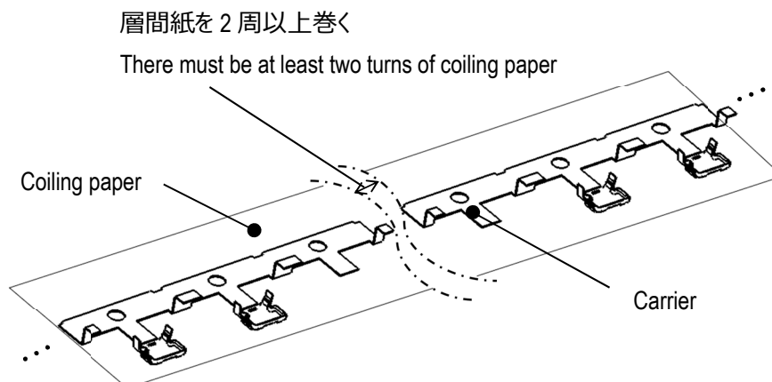
Fig.3 Connection of carrier
